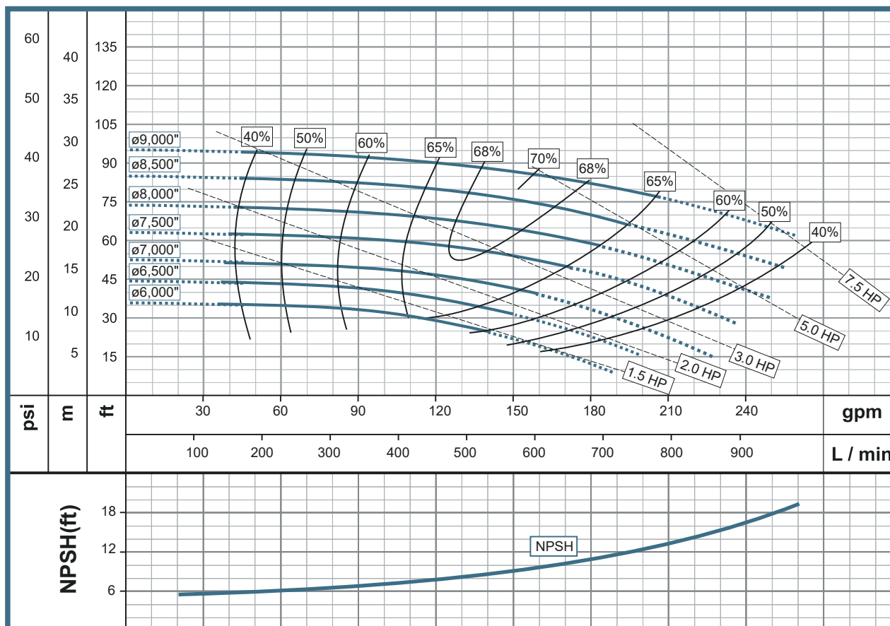
Performance Curve
