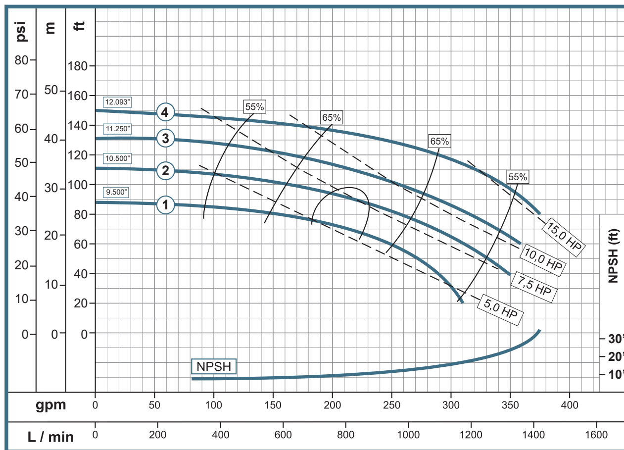
Performance Curve
