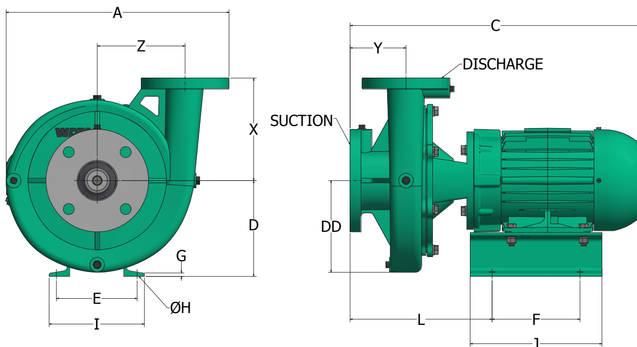
QE (B) - Dimensions (inches)
