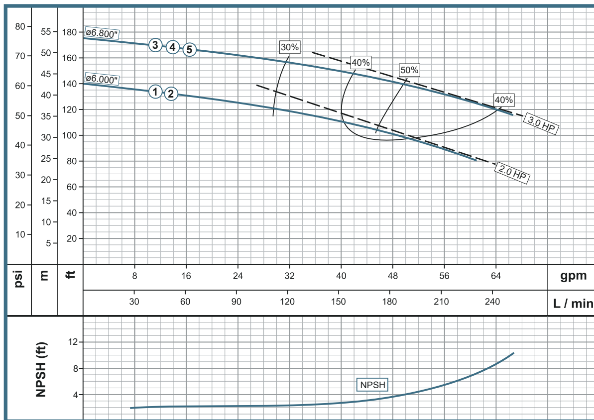
Performance Curve
