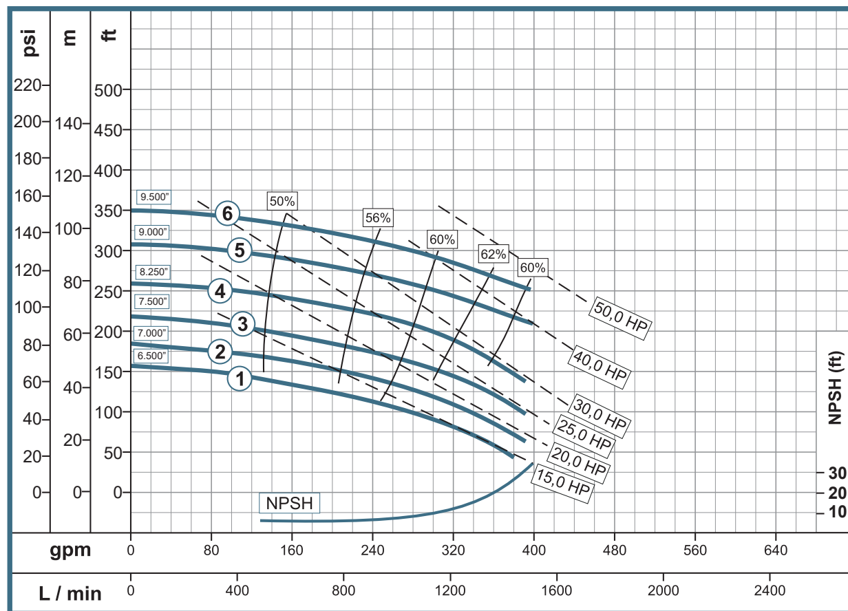
Performance Curve
