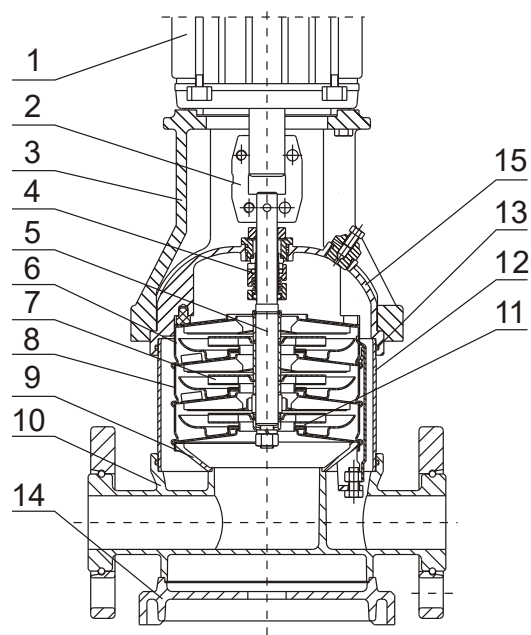
VSSE PUMP
